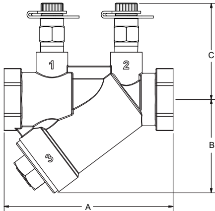
Model AL illustration and Nominal Dimensions shown with two optional "PL" Low-Lead Pressure/ Temperature Test Ports
